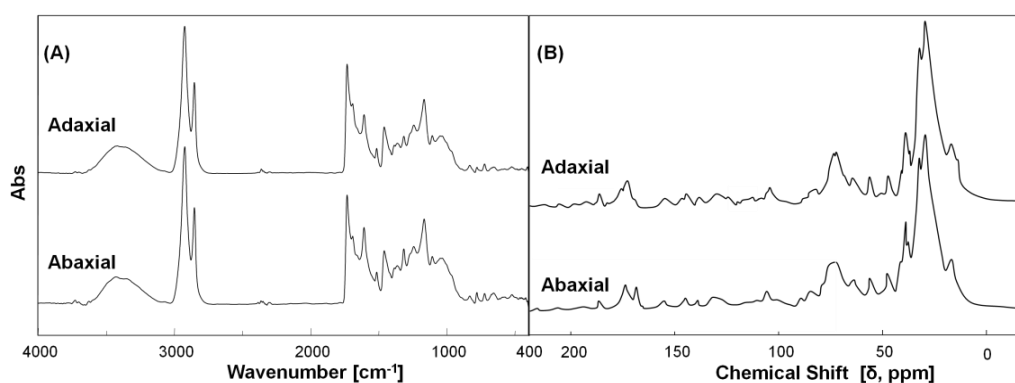
Figure 2. Typical (A) FT-IR spectra and (B) solid-state CP/MAS ^{13}\text{C} NMR spectra of the CMs isolated from young matured leaves ( L_3 ) of S. alba .
